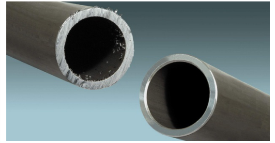
Application: clean internal and external deburring of steel pipes after cutting.
